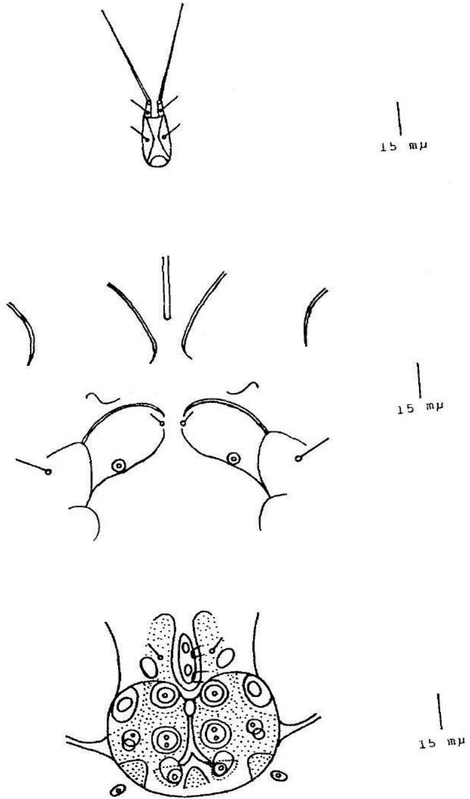
Figs. 3, Gnathosoma (upper), Coxal apodemes (middle), Suctorial shield (lower) of C. arbelos n. sp.
