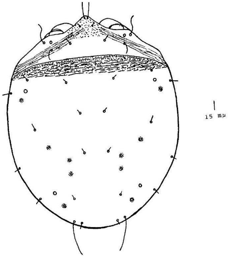
Fig. 1 showing Dorsal view of C. arbelos n. sp.
