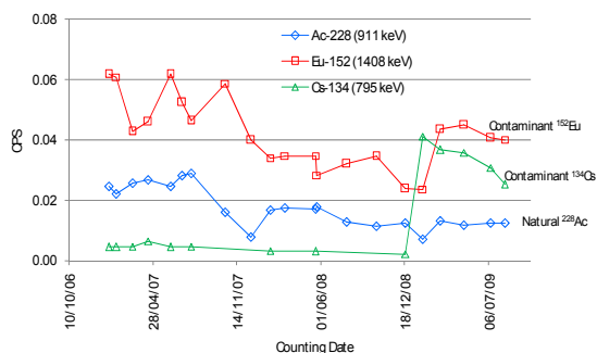
Figure 6. A comparison of count rates of 1408 keV peak of ^{152}\text{Eu} , 795 keV peak of ^{134}\text{Cs} and 911 keV peak of ^{228}\text{Ac} .
