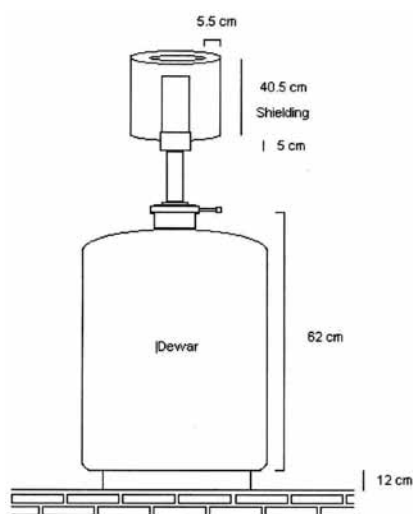
Figure 1. Housing of HPGe detector with shielding, the dimensions are not to the scale.
