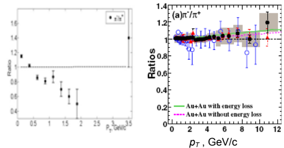
Figure 2. The \pi^-/\pi^+ ratios in: (left) \pi^-^{12}\text{C} interactions at 40GeV/c; (right) 12% central ( \circ ), MB \text{Au}+\text{Au} ( \bullet ) and d+\text{Au} ( \blacktriangle ) [24] collisions at \sqrt{s_{\text{NN}}}=200\text{GeV} .
