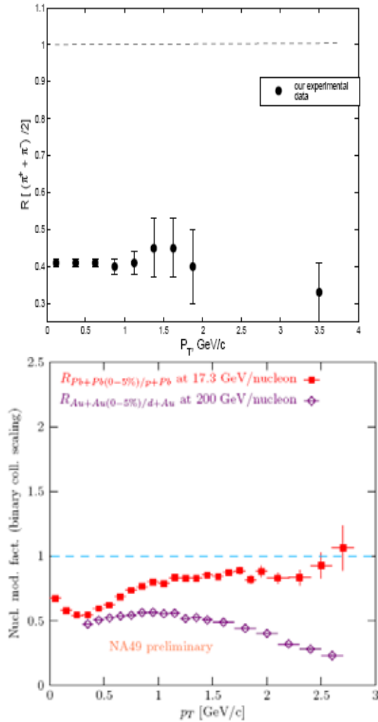
Figure 3. The (\pi^+ + \pi^-)/2 R(p_T) dependence in different collisions.
