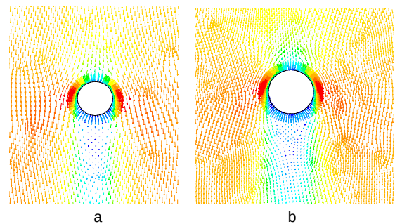
Figure 6. Velocity vectors around bubbles with unstructured mesh (a) 1.0 mm dia.; (b) 1.5 mm dia.
