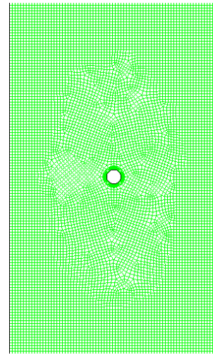
Figure 2. Schematic diagram of geometry for bubble of 1.0mm diameter with unstructured mesh.
