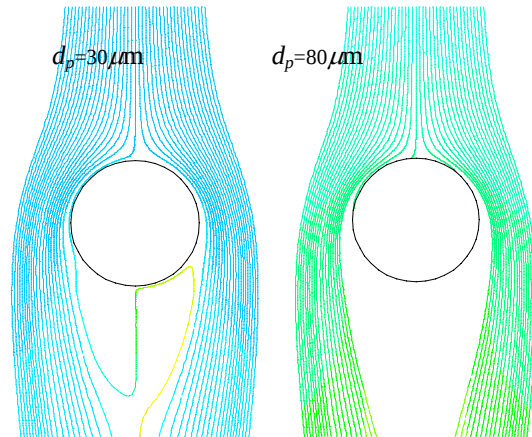
Figure 9. Tracks of particle streamlines around 1.5 mm diameter bubble with unstructured mesh.
