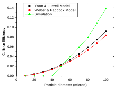
Figure 12. Comparison of the results of CFD simulations and hydrodynamic models for 1.0 mm bubble with unstructured mesh geometry.
