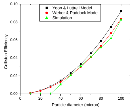
Figure 14. Comparison of the results of CFD simulations and hydrodynamic models for 1.0 mm bubble with structured mesh geometry.
