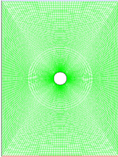
Figure 4. Schematic diagram of geometry for bubble of 1.0 mm diameter with structured mesh.
