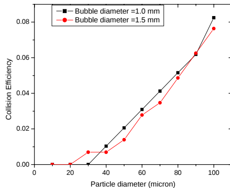
Figure 16. Comparison of collision probabilities for different bubble diameters with structured mesh geometry.
