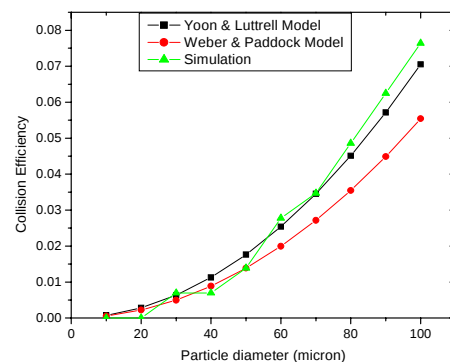
Figure 15. Comparison of the results of CFD simulations and hydrodynamic models for 1.5 mm bubble with structured mesh geometry.
