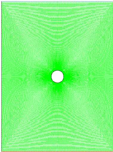
Figure 5. Schematic diagram of geometry for bubble of 1.5 mm diameter with structured mesh.
