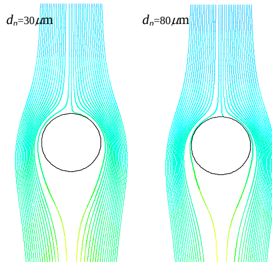
Figure 10. Tracks of particle streamlines around 1.0 mm diameter bubble with structured mesh.
