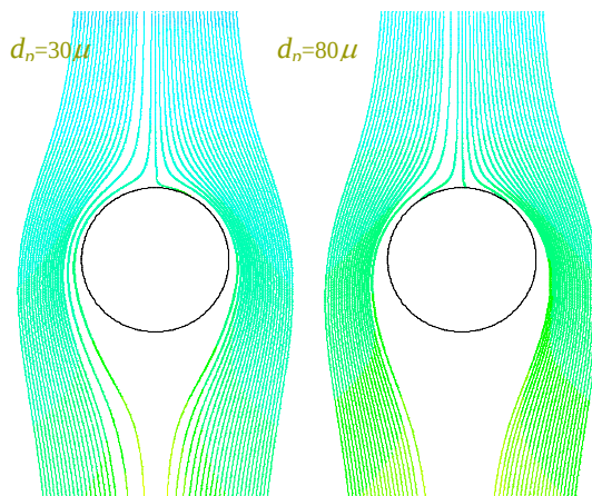
Figure 11. Tracks of particle streamlines around 1.5 mm diameter bubble with structured mesh.
