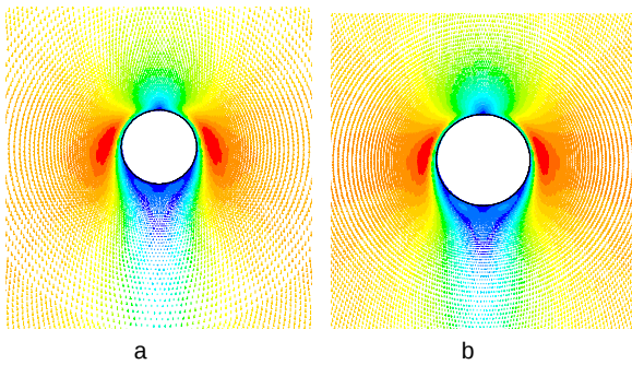
Figure 7. Velocity vectors around bubbles with structured mesh (a) 1.0 mm dia.; (b) 1.5 mm dia.
