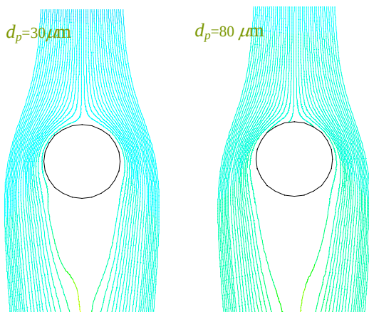
Figure 8. Tracks of particle streamlines around 1.0 mm diameter bubble with unstructured mesh.
