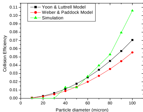
Figure 13. Comparison of the results of CFD simulations and hydrodynamic models for 1.5 mm bubble with unstructured mesh geometry.
