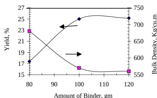
Figure 8. Effect of amount of binder on yield and bulk density.
