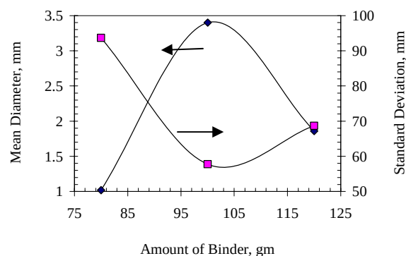
Figure 9. Effect of amount of binder used on mean diameter ( d_{50} ) and standard deviation.
