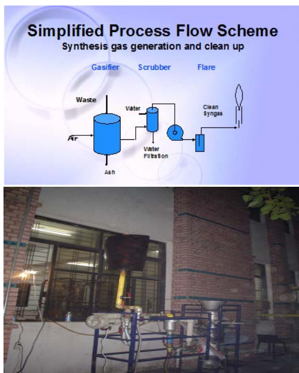
Figure 1. Process diagram and Picture Plate.
