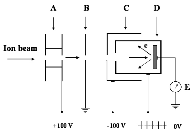
Figure 1. Schematic diagram of the experimental setup used for secondary electron emission studies. (A) Beam defining collimator, (B) Stripping aperture, (C) rejection aperture, (D) cage and (E) Pico-Ampere meter.
