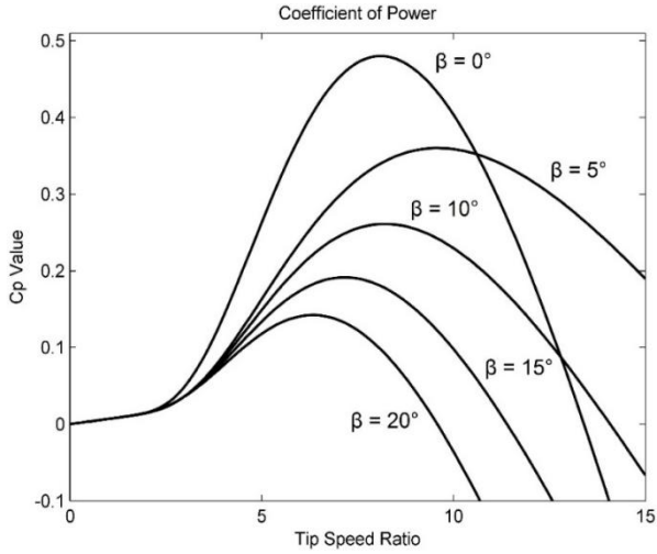
Figure 1. C_p Characteristics
