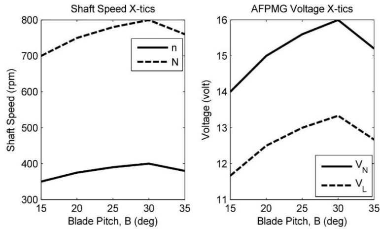
Figure 11. WES model results on variable B.
