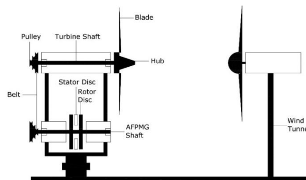
Figure 1. Proposed layout of micro WES model.
