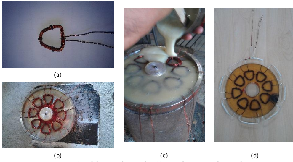
Figure 6. (a) Coil (b) Stator disc template (c) Stator disc casting, (d) Stator disc.
