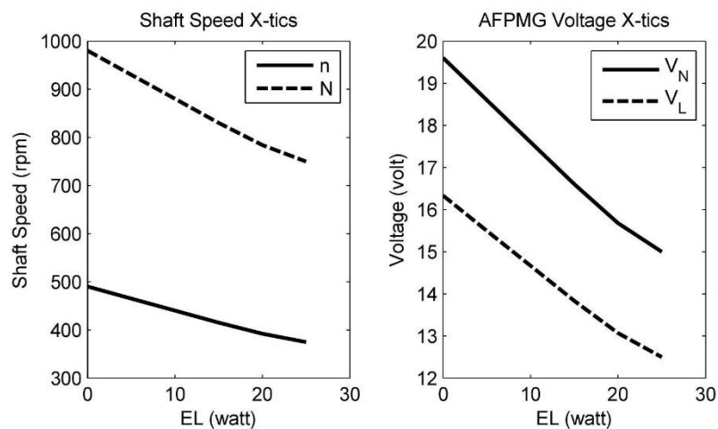
Figure 13. WES model results on variable EL.
