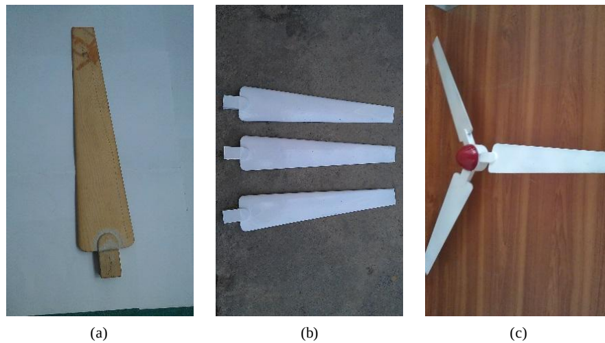
Figure 4. (a) Wooden blade pattern, (b) Aluminium casted blades, (c) Propeller of wind turbine.
