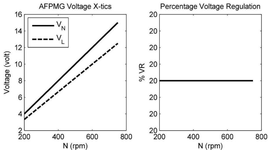
Figure 14. Voltage regulation of AFPMG.
