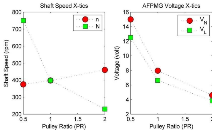
Figure 12. WES model results on variable PR
