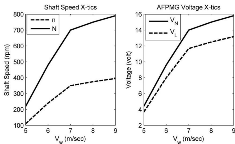
Figure 10. WES model results on variable V_w
