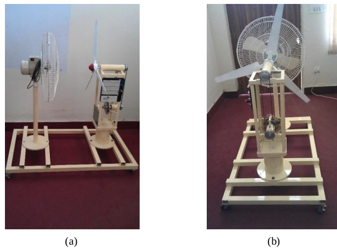
Figure 8. Complete micro WES model.
