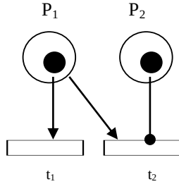
Figure 6. Priority in Petri nets.
