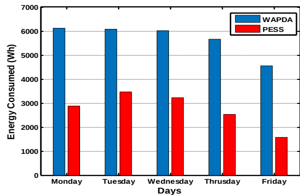
Fig. 7: Energy consumption per day in UET Library
