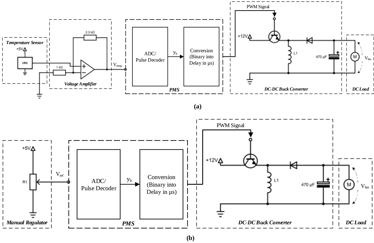
Fig. 5: Block diagram of fan control system (a) automatic (b) manual
