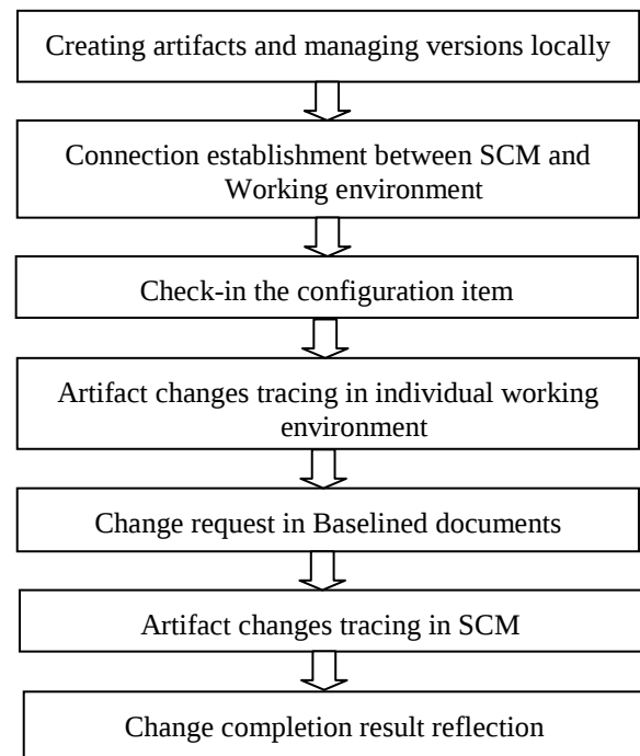
Fig. 2: Change management process in SCM and the working environment
