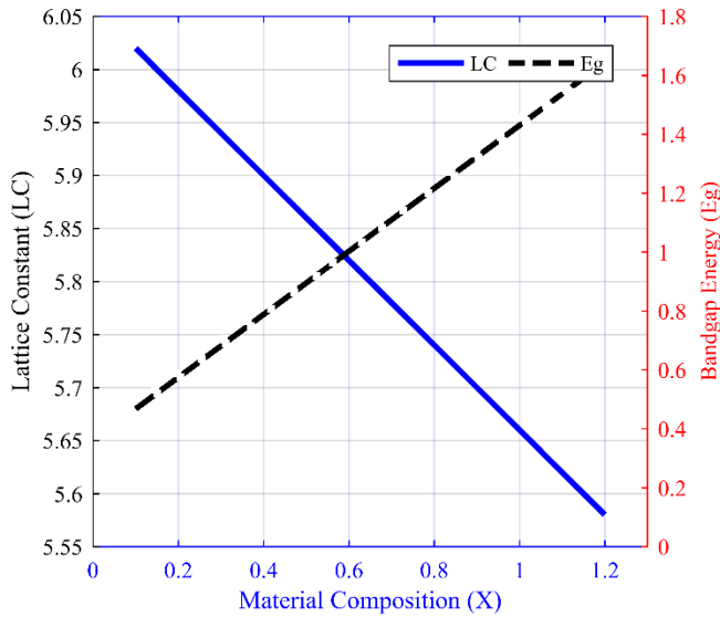
Fig. 2: E_g and LC for different compositions (X) of \text{In}_{1-X}\text{Ga}_X\text{As} .
