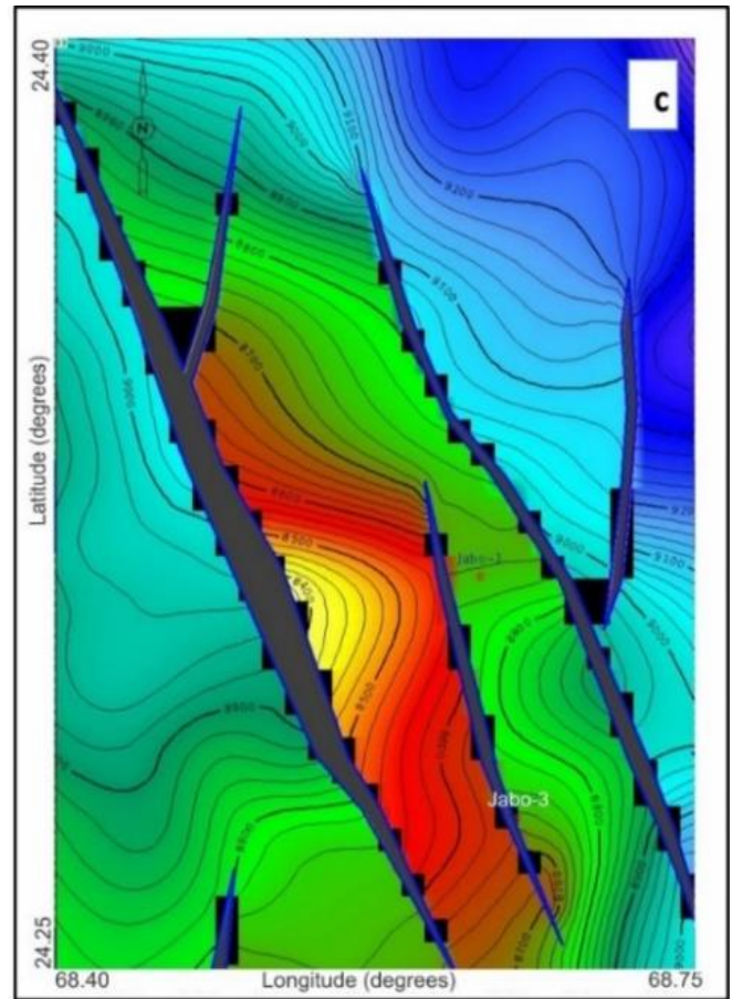
Fig. 5: Depth structure maps of (a) Top Lower Goru (TLG), (b) Top Middle Sand (TMS) and (c) Top Basal Sand level (TBSL). The values are shown in feet.
