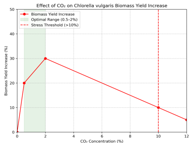
Fig. 4 Chlorella vulgaris yield peaked at 0.5-2% CO 2 , while >10% reduced growth [29, 43, 44].
