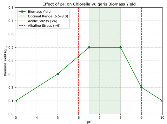
Fig. 3 Effect of pH on Chlorella vulgaris biomass yield. Maximum growth occurred within the optimal pH range (6.5-8.0), while acidic (<6) and alkaline (>9) stress reduced yield [21, 28].
