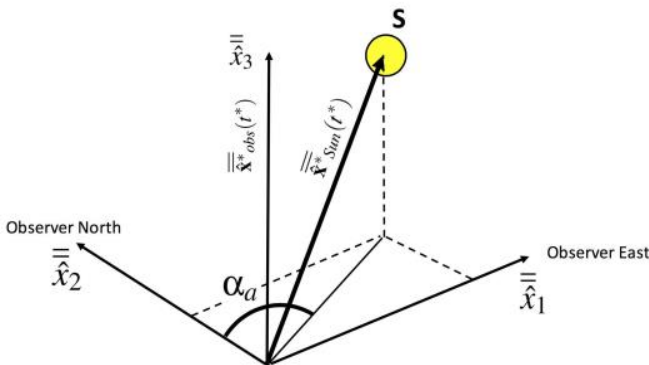
Fig. 5 The observer position vector \bar{\bar{x}}_{obs}^*(t^*) , the Sun position vector \bar{\bar{x}}_{Sun}^*(t^*) and the solar azimuth angle measured from north \alpha_a in the Cartesian coordinate system o, \bar{\bar{x}}_1, \bar{\bar{x}}_2, \bar{\bar{x}}_3 . The observer horizon plane is defined by the plane \bar{\bar{x}}_1 - \bar{\bar{x}}_2 , where \bar{\bar{x}}_1 is the observer's East while \bar{\bar{x}}_2 is the observer North.
