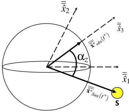
Fig. 4 The observer position vector \bar{\bar{x}}_{obs}^*(t^*) , the Sun position vector \bar{\bar{x}}_{Sun}^*(t^*) and the solar zenith angle \alpha_z in the Cartesian coordinate system o, \bar{\bar{x}}_1, \bar{\bar{x}}_2, \bar{\bar{x}}_3 .
