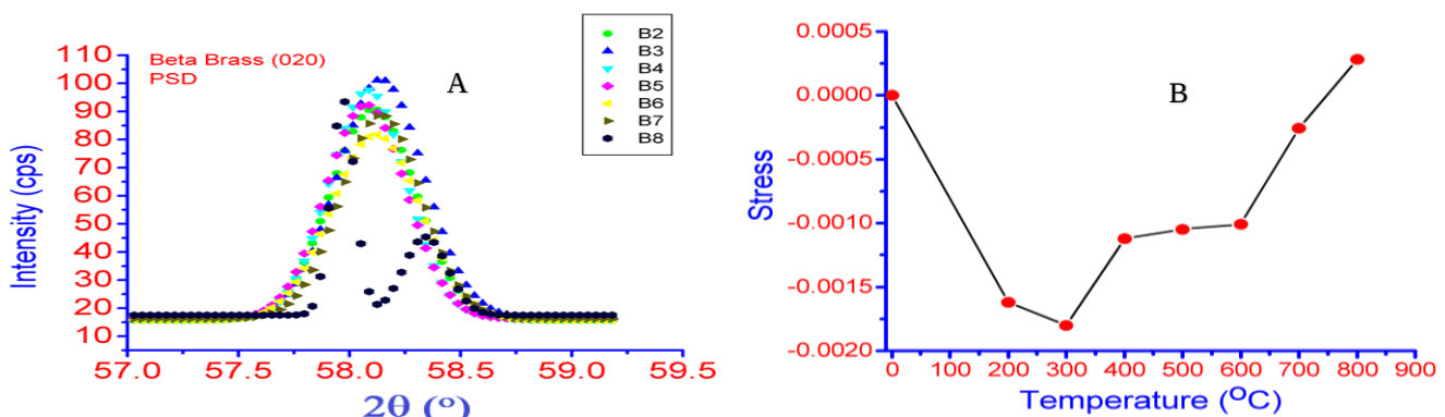
Fig. 1: (A) Change in the 2\theta position of Bragg peaks in brass sample measured at different temperatures, (B) calculated residual stress as a function of temperature.
