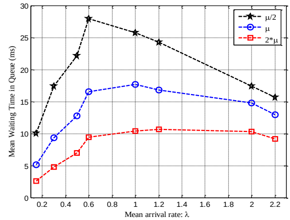
Fig. 10: Mean waiting time in queue versus arrival rate with the security off at different values of \mu .
